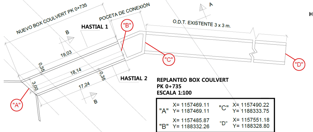
Box culvert 3*3
